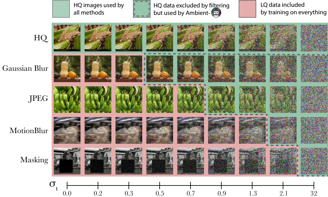
Figure 3: Visual summary of our method for using low-quality data at high-noise. We see how the various corrupted images become indistinguishable from the High Quality (HQ) after a minimum noise level. These noisy versions of Low Quality (LQ) images are actually high-quality data, which filtering approaches discard, but Ambient Omni uses.
