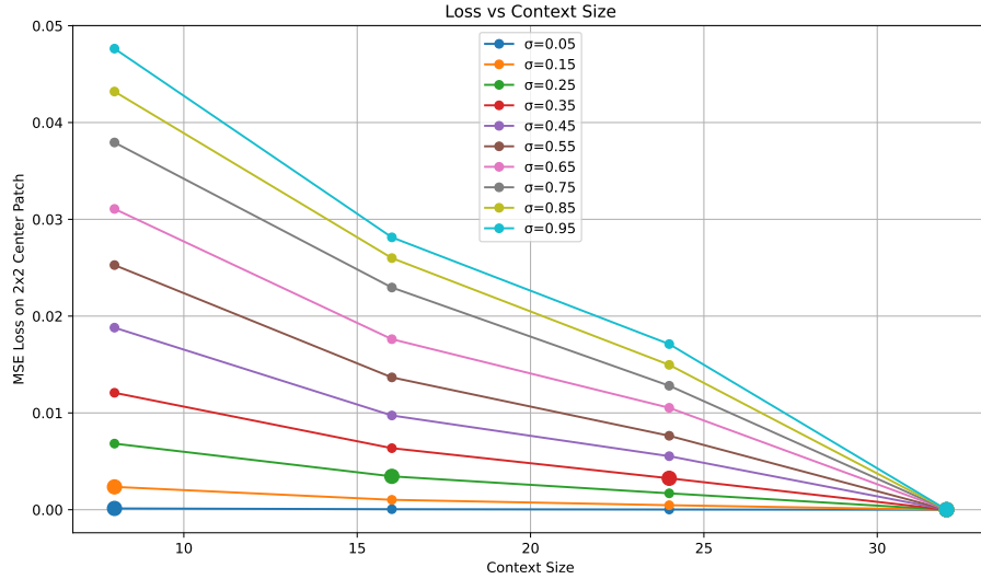
Figure 15: ImageNet-512x512: denoising loss of an optimally trained model, measured at 2 \times 2 center patch, as we increase the context size given to the model (horizontal axis) and the noise level (different curves). As expected, for higher noise, more context is needed for optimal denoising. The large dot on each curve marks the point where the loss nearly plateaus.
